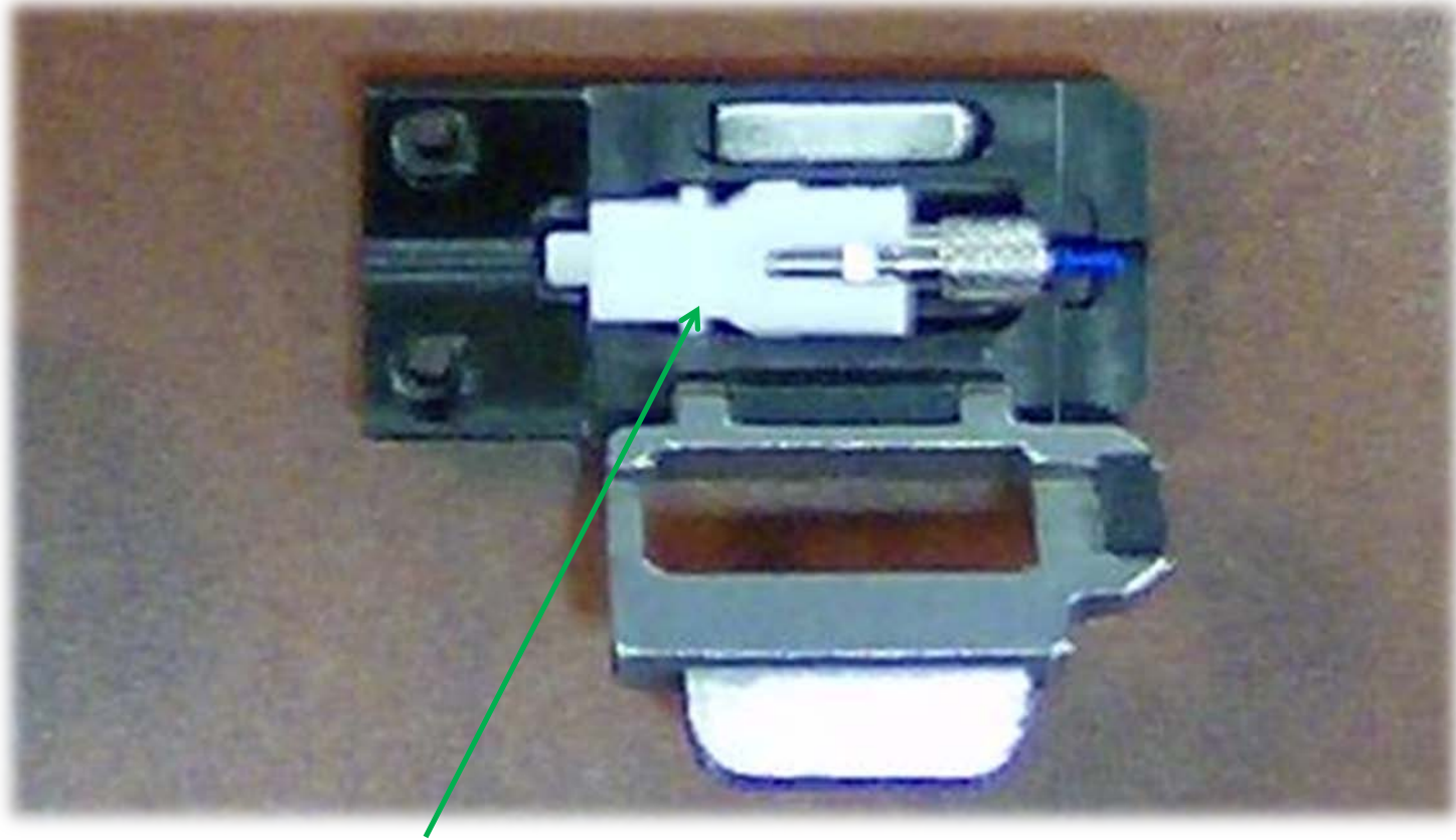
SC/LC adapter with SC/UPC SOC installed
