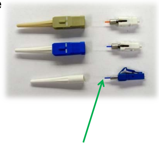
Factory cleaved fiber stub
