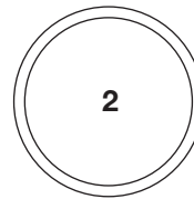
50420891 I.D. = .787 O.D. = .889
